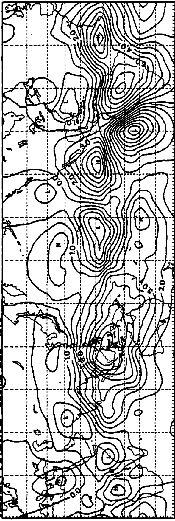
VELOCITY POTENTIAL 200MB DEC 1975
